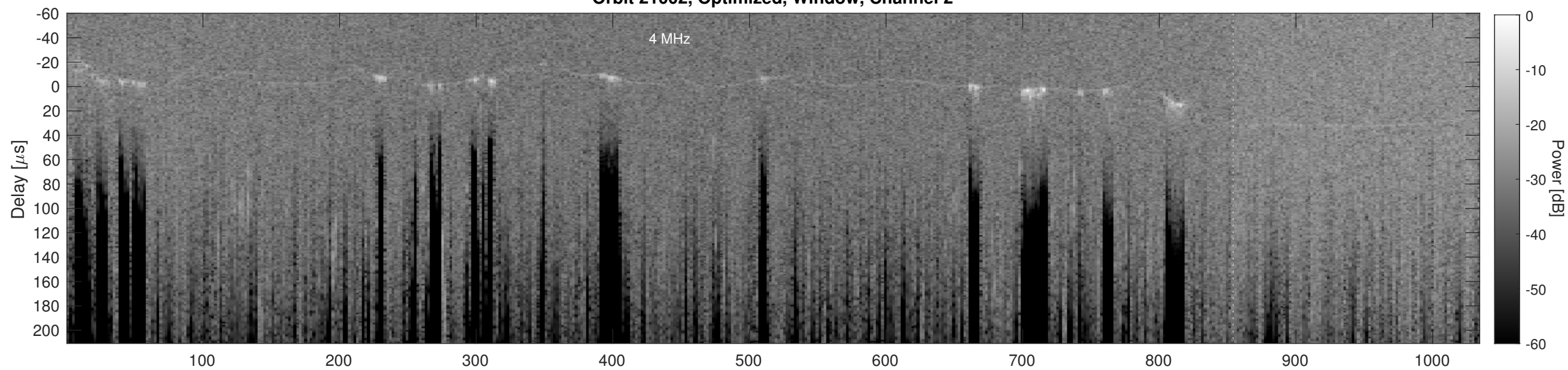
Orbit 21002, Cluttergram
