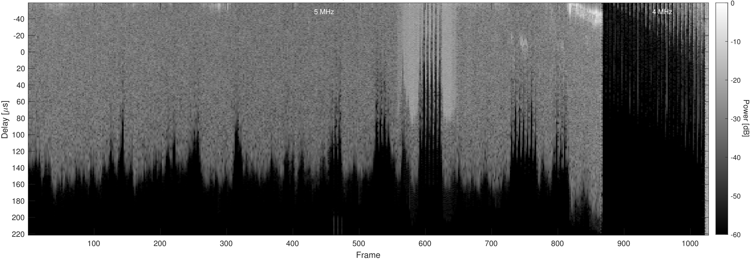
Orbit 21004, Chapman, No Window, Channel 2
