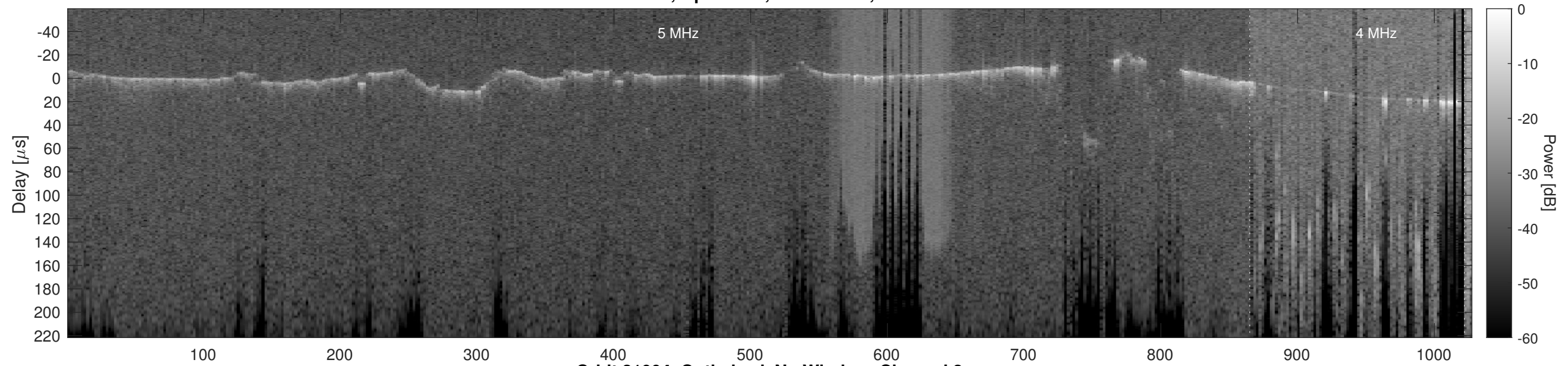
Orbit 21004, Optimized, No Window, Channel 2
