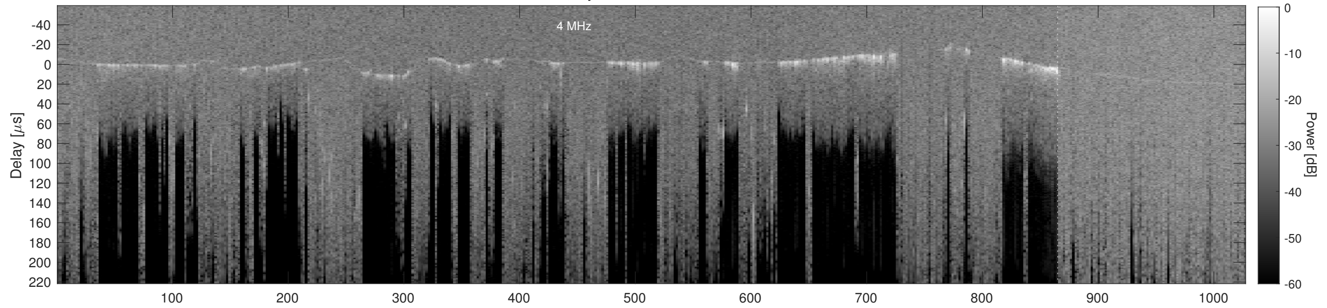
Orbit 21004, Cluttergram
