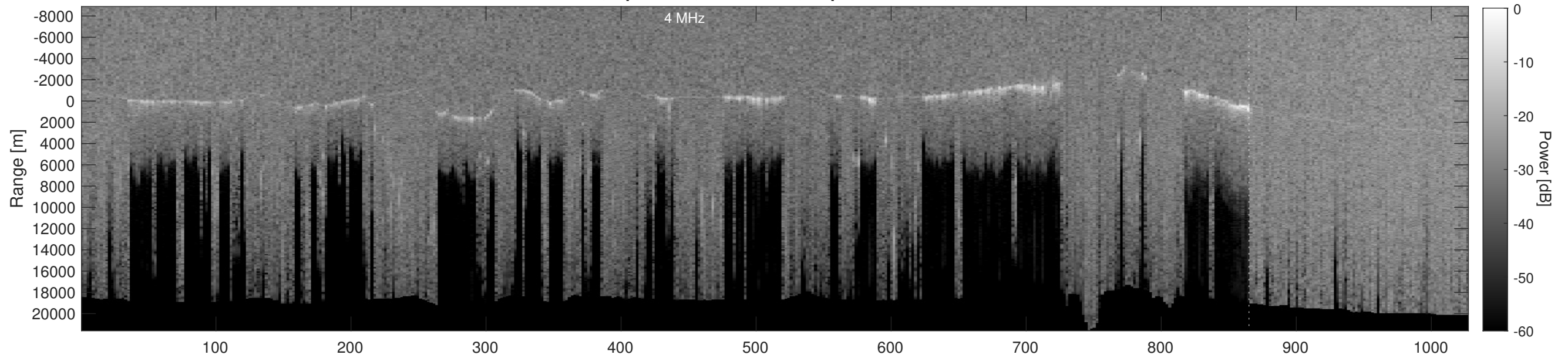
Orbit 21004, Depth-Corrected Cluttergram
