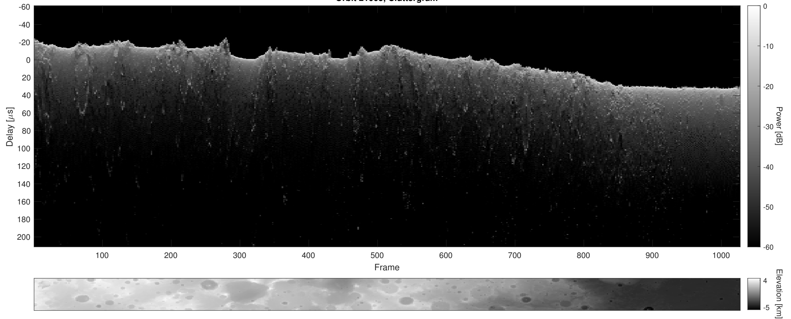
Orbit 21005, Cluttergram
