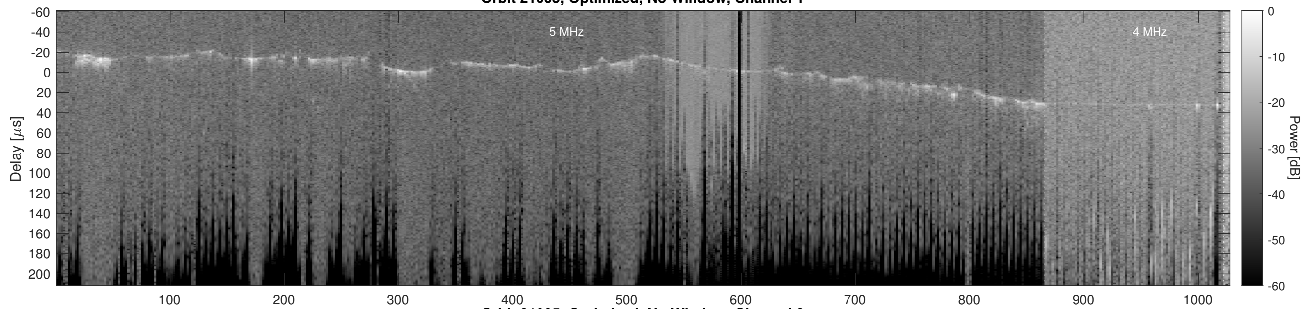
Orbit 21005, Optimized, No Window, Channel 2
