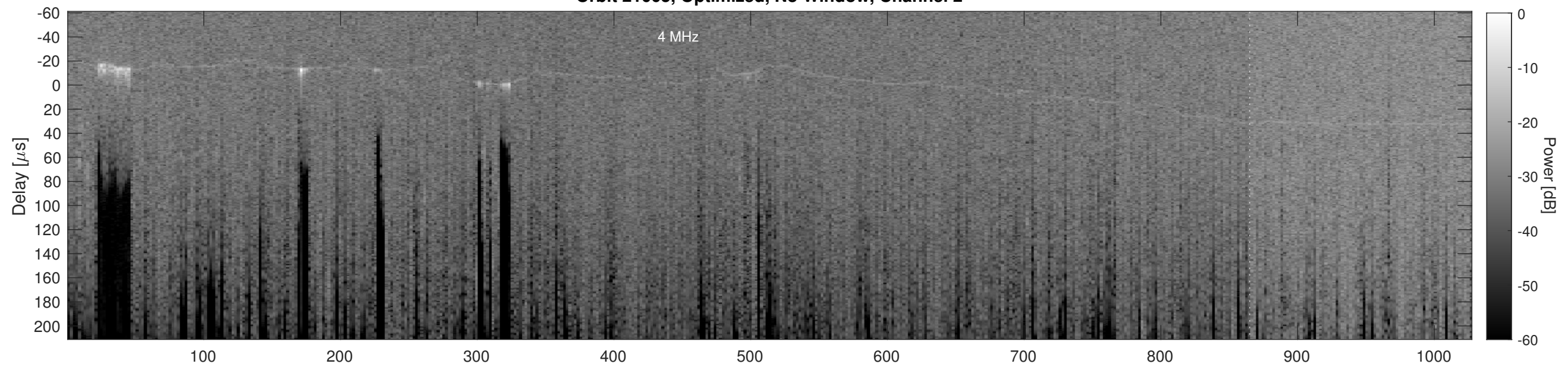
Orbit 21005, Cluttergram
