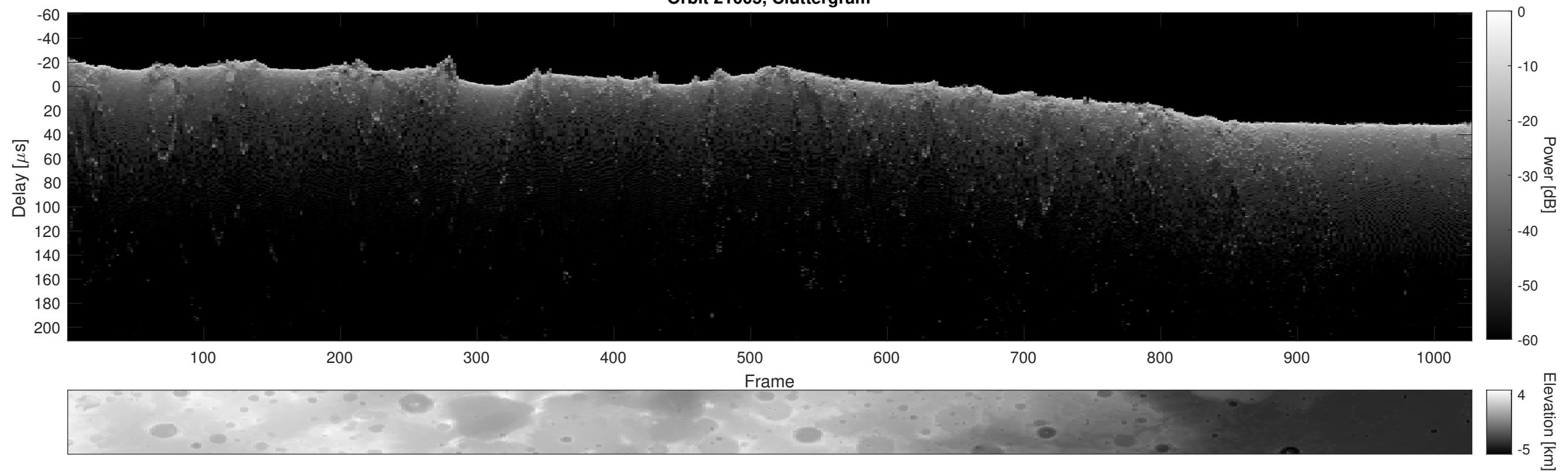
Orbit 21005, Cluttergram
