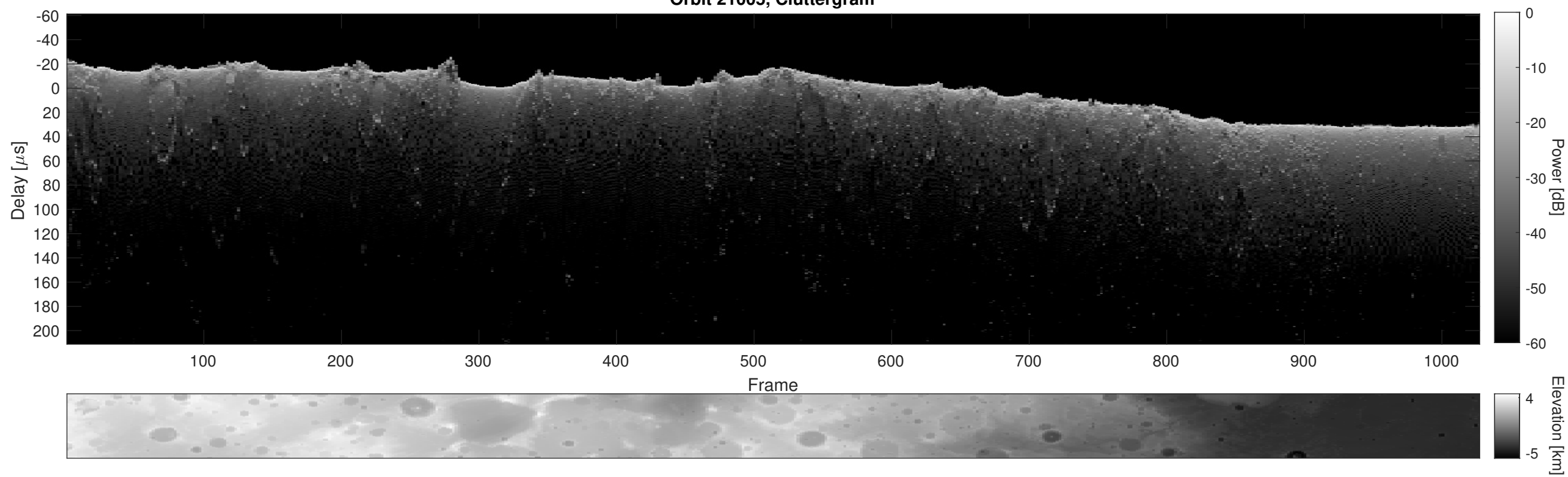
Orbit 21005, Cluttergram
