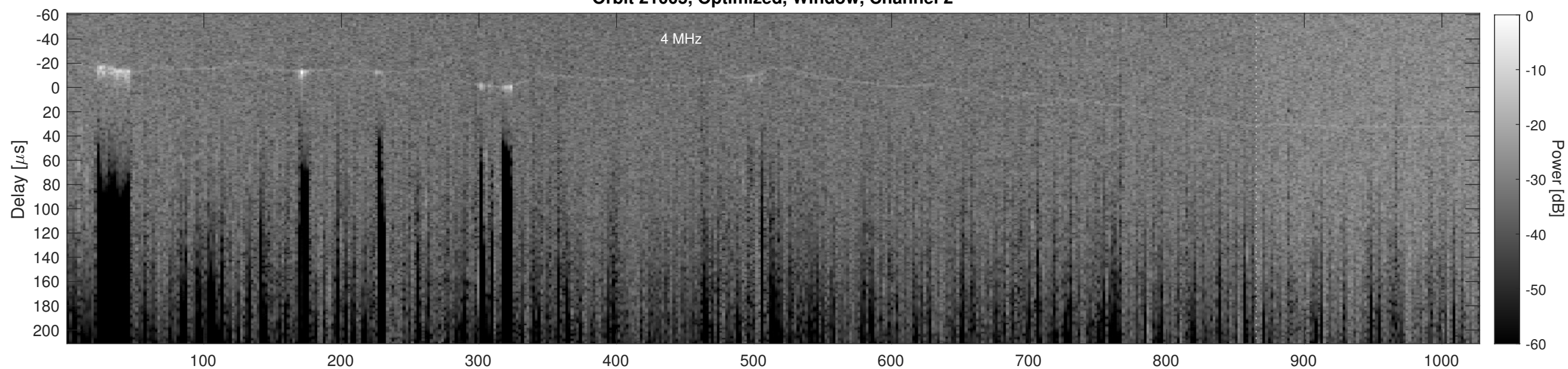
Orbit 21005, Cluttergram
