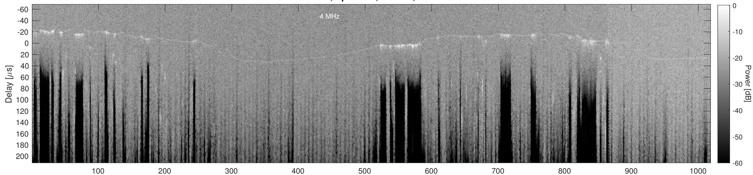
Orbit 21006, Cluttergram
