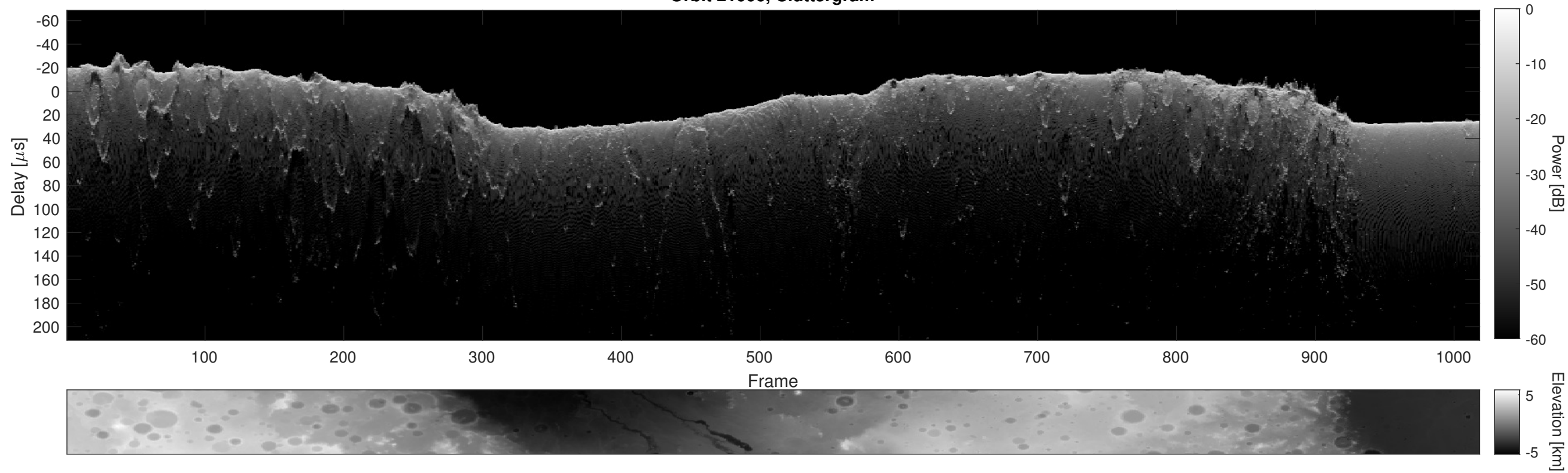
Orbit 21006, Cluttergram
