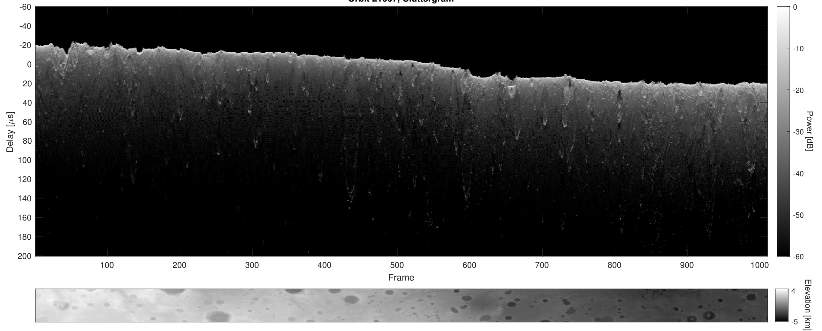
Orbit 21007, Cluttergram
