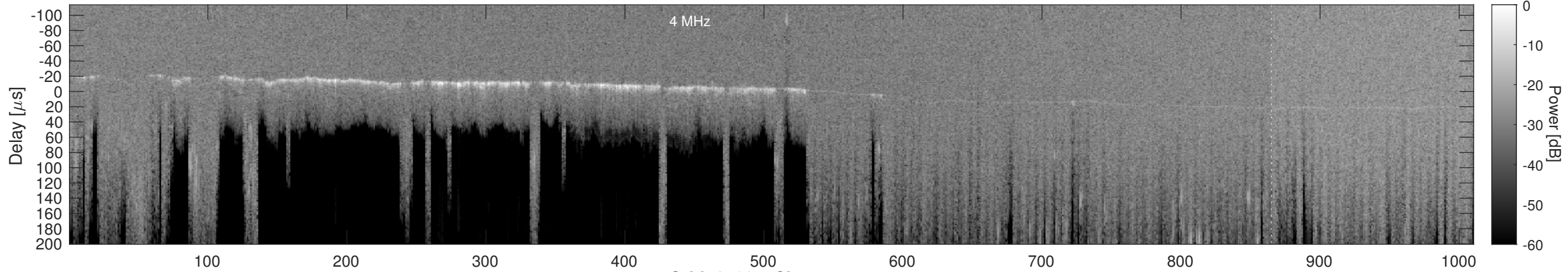
Orbit 21007, Cluttergram
