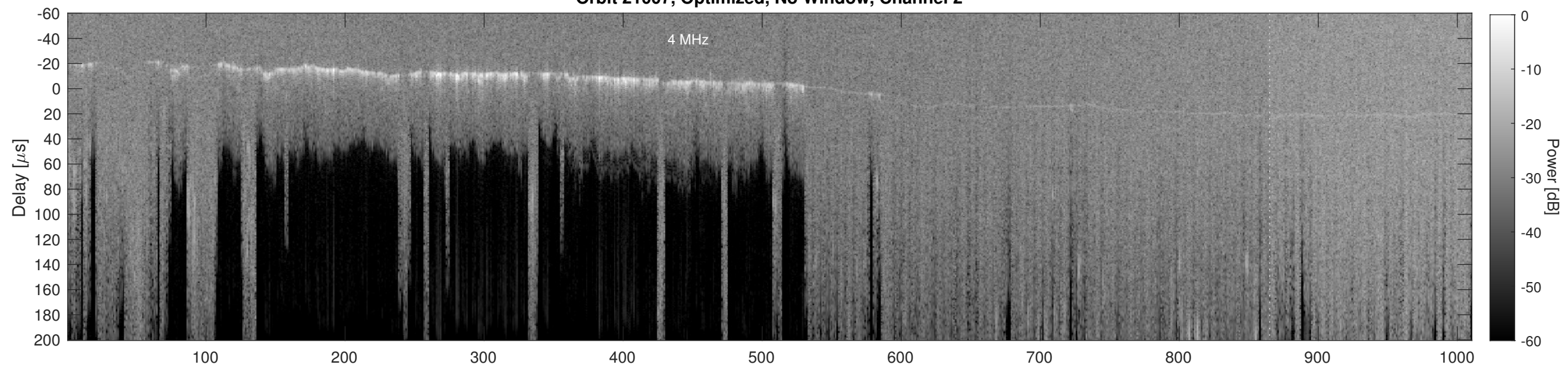
Orbit 21007, Cluttergram
