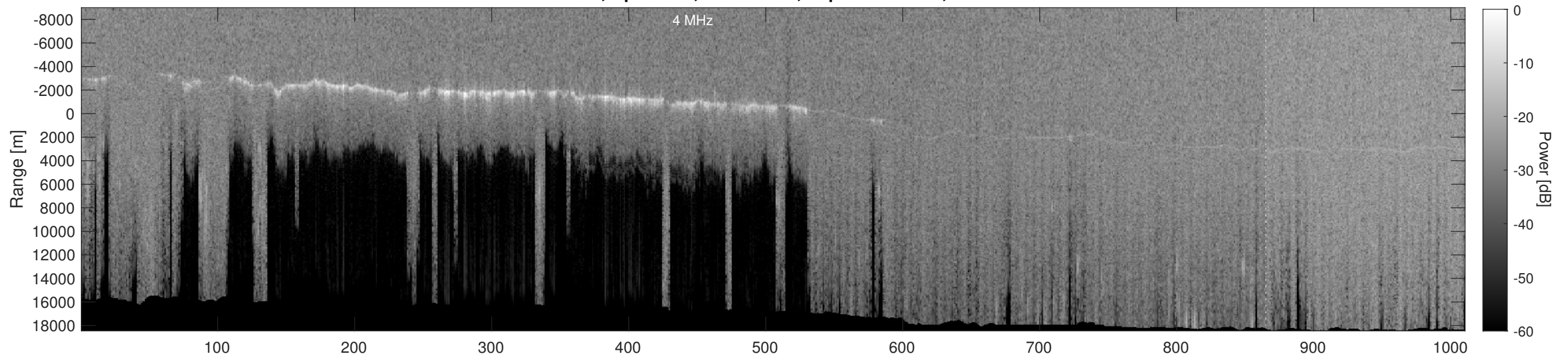
Orbit 21007, Depth-Corrected Cluttergram
