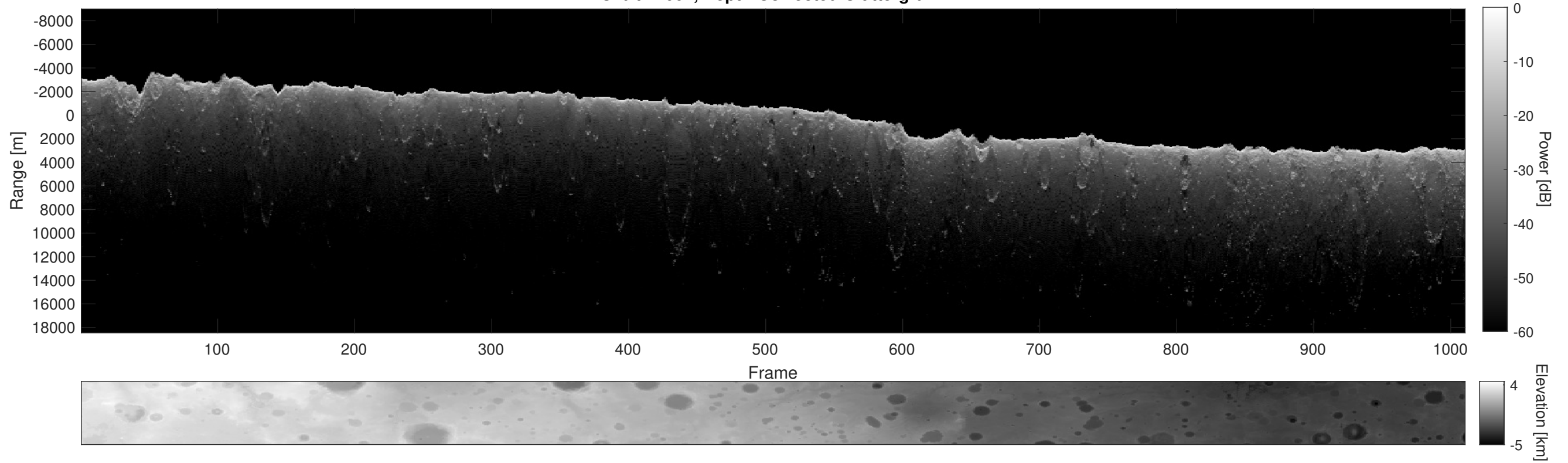
Orbit 21007, Depth-Corrected Cluttergram
