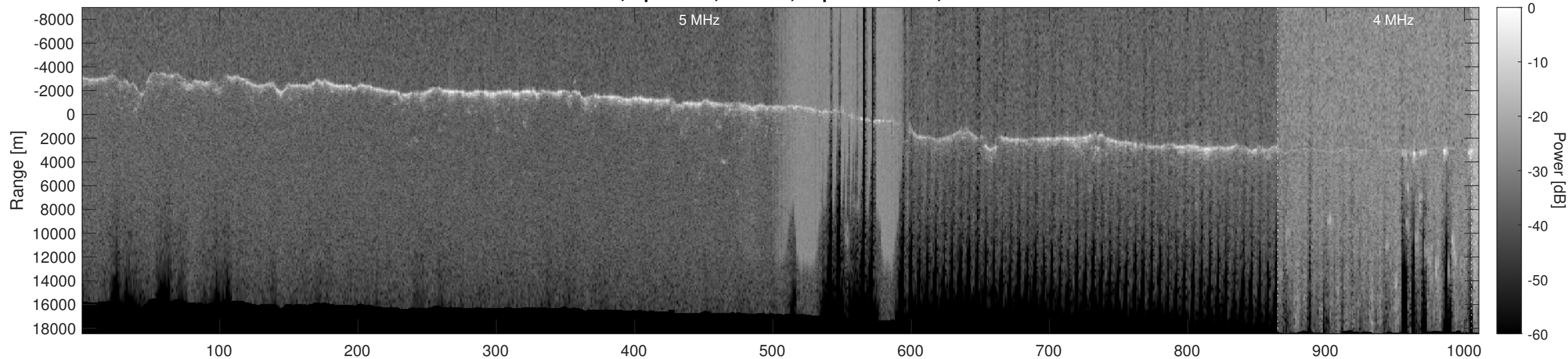
Orbit 21007, Optimized, Window, Depth-Corrected, Channel 2
