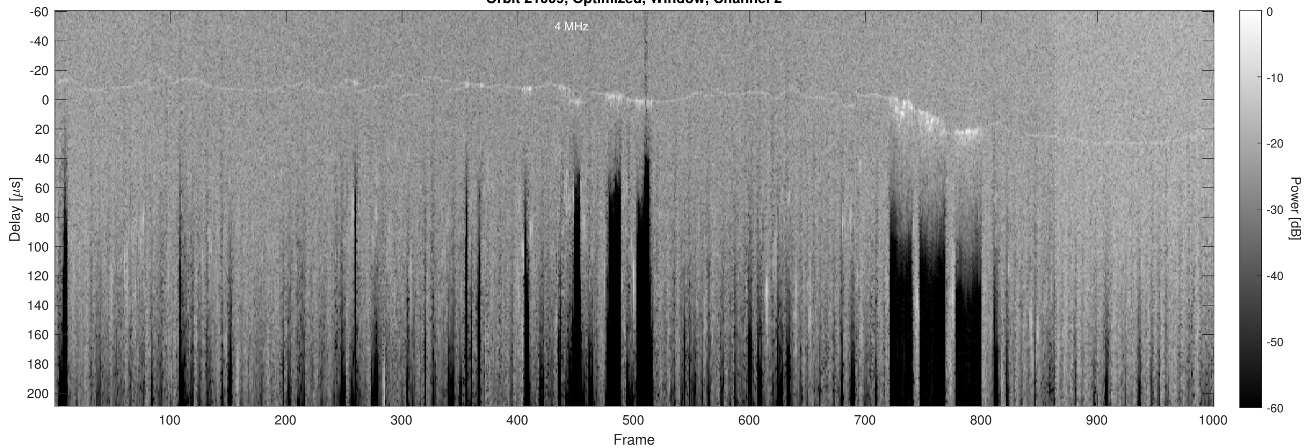
Orbit 21009, Optimized, Window, Channel 2
