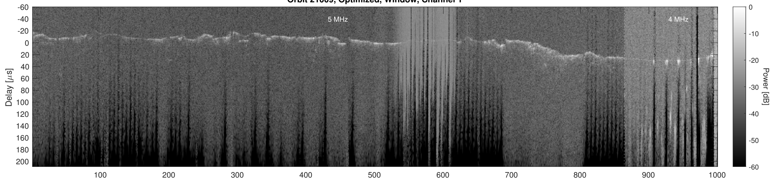
Orbit 21009, Optimized, Window, Channel 2
