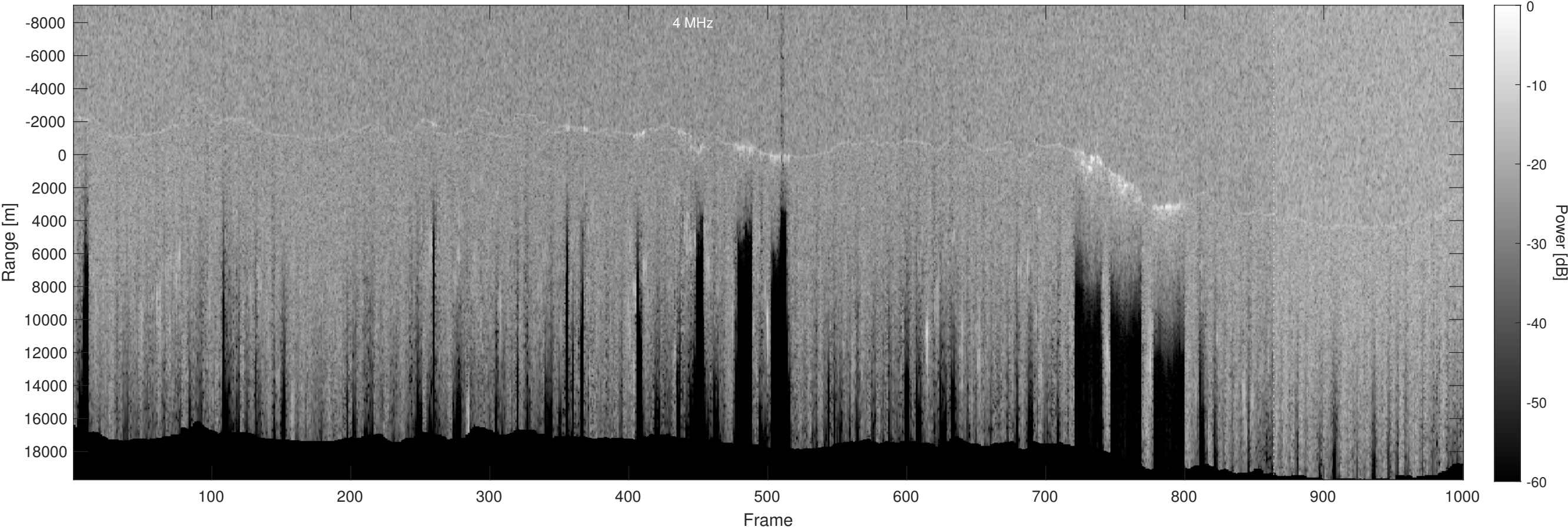
Orbit 21009, Optimized, Window, Depth-Corrected, Channel 2
