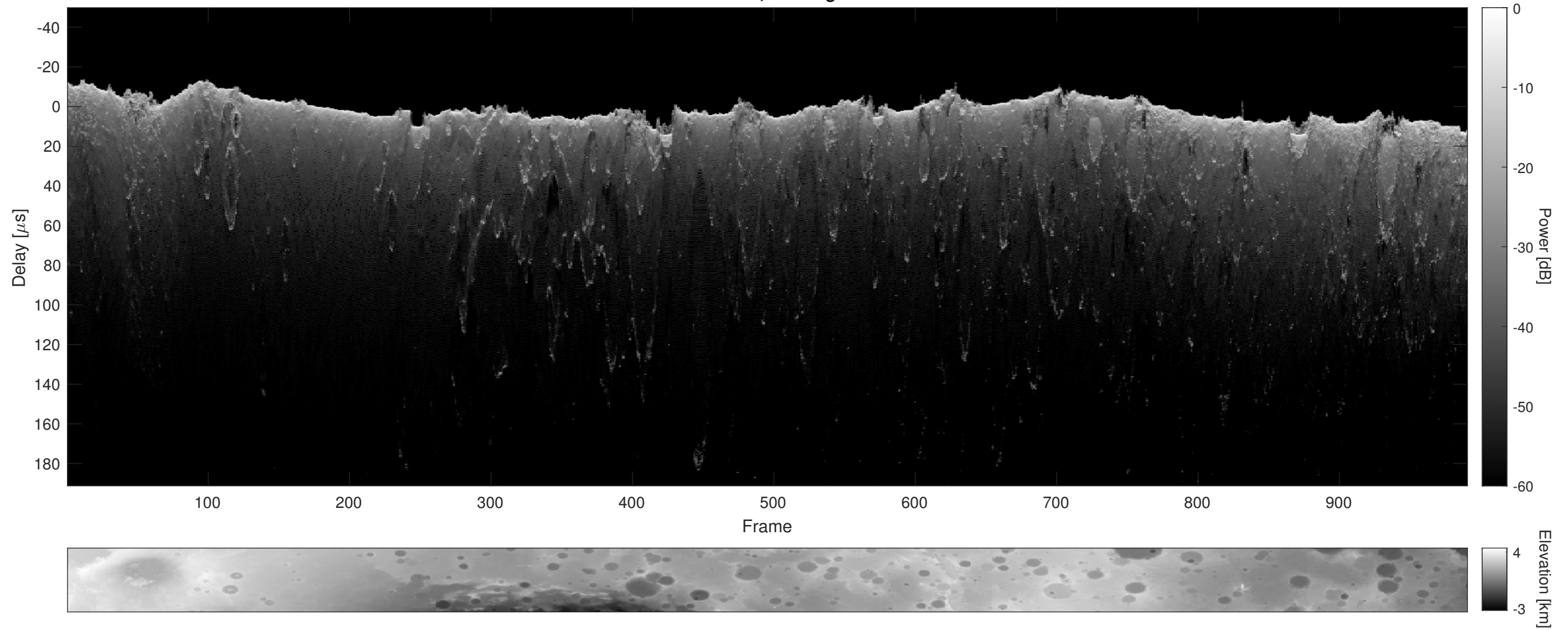
Orbit 21010, Cluttergram
