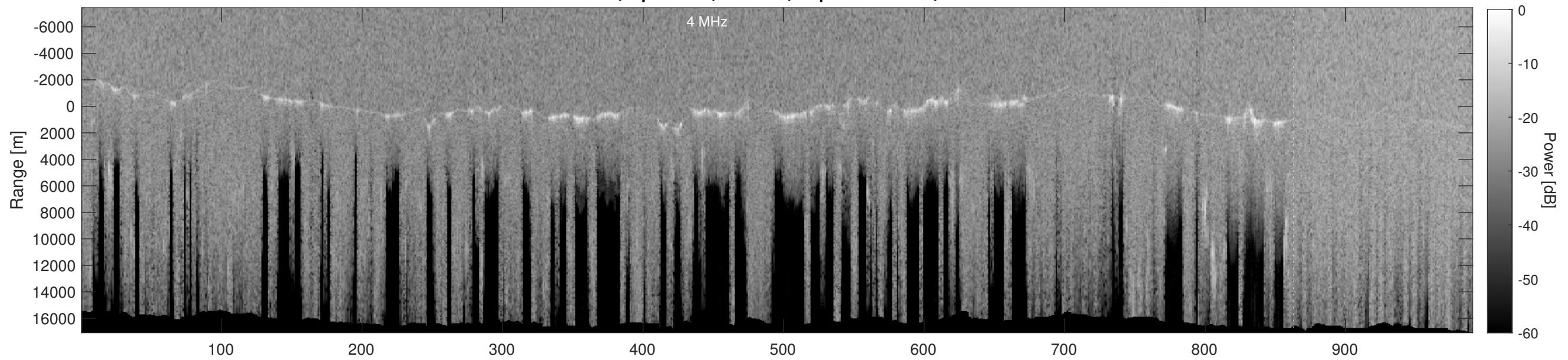
Orbit 21010, Depth-Corrected Cluttergram
