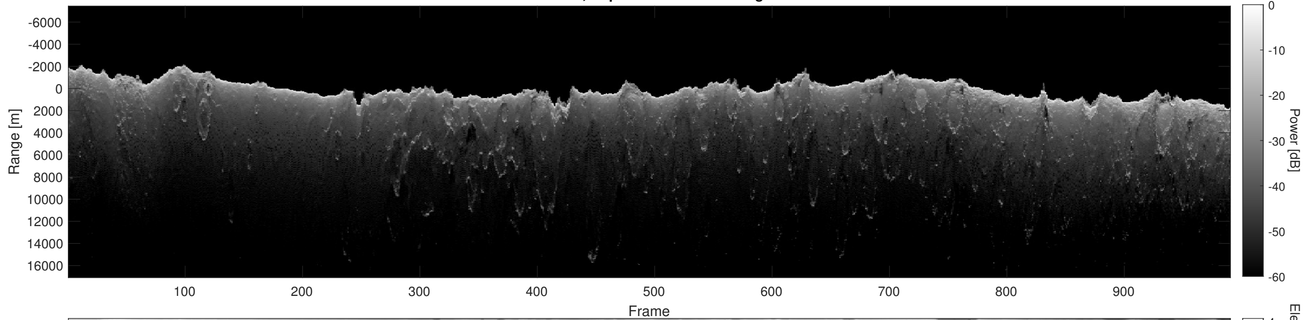
Orbit 21010, Depth-Corrected Cluttergram
