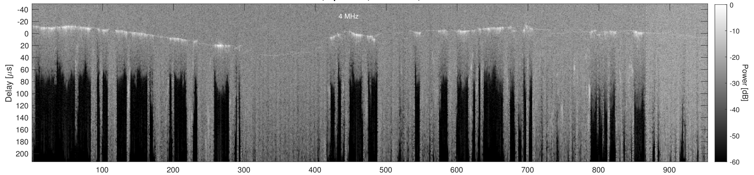
Orbit 21017, Cluttergram
