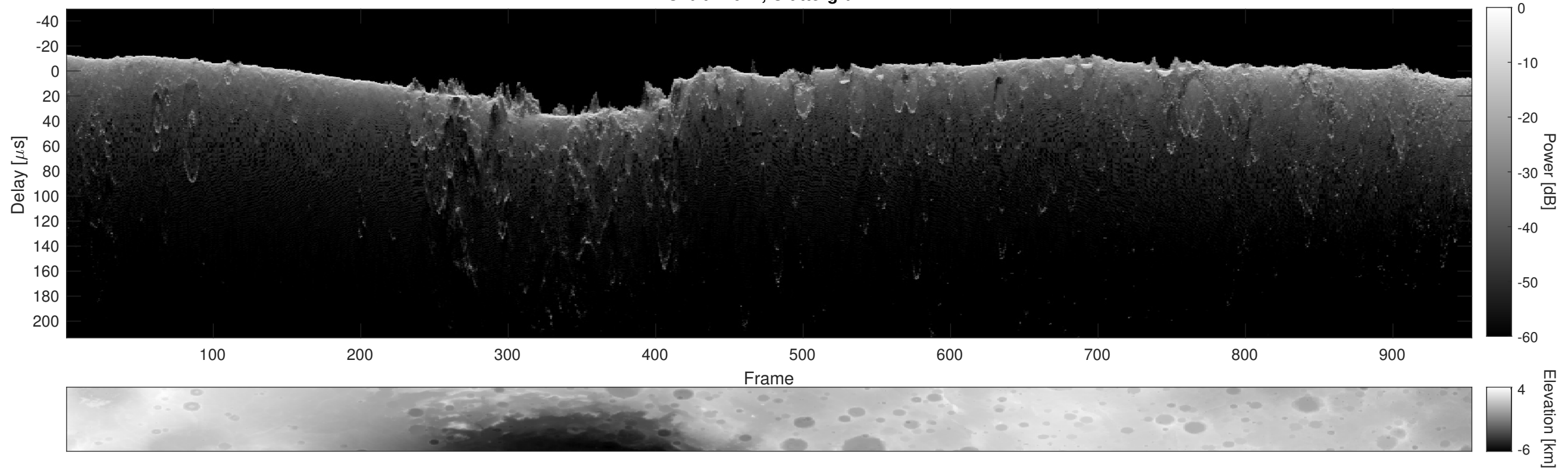
Orbit 21017, Cluttergram
