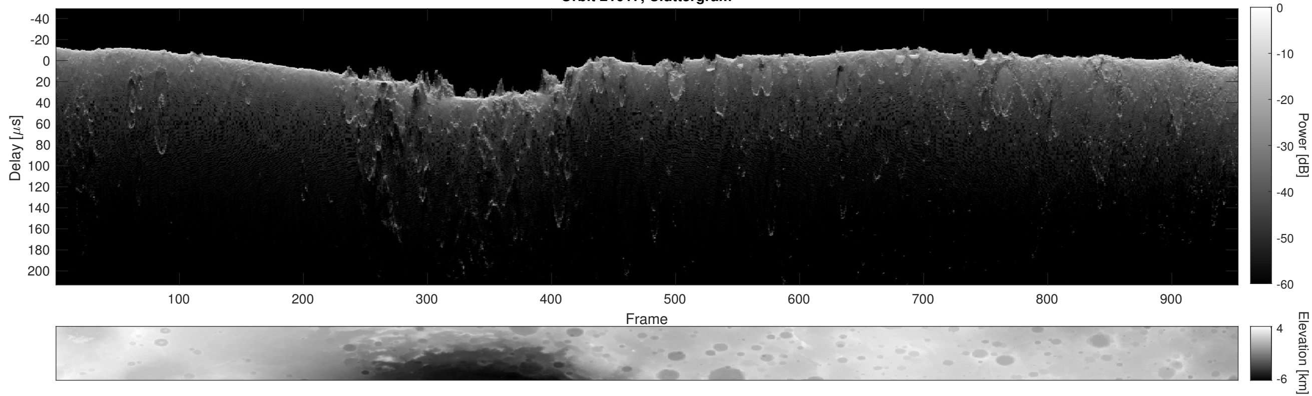
Orbit 21017, Cluttergram
