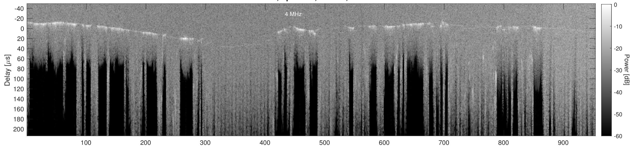
Orbit 21017, Cluttergram
