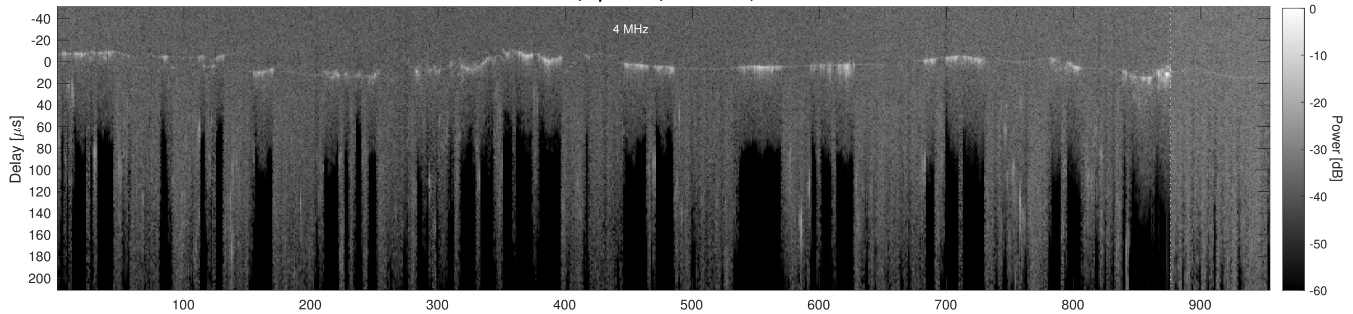
Orbit 21018, Cluttergram
