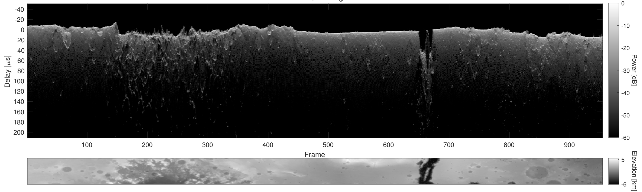
Orbit 21018, Cluttergram
