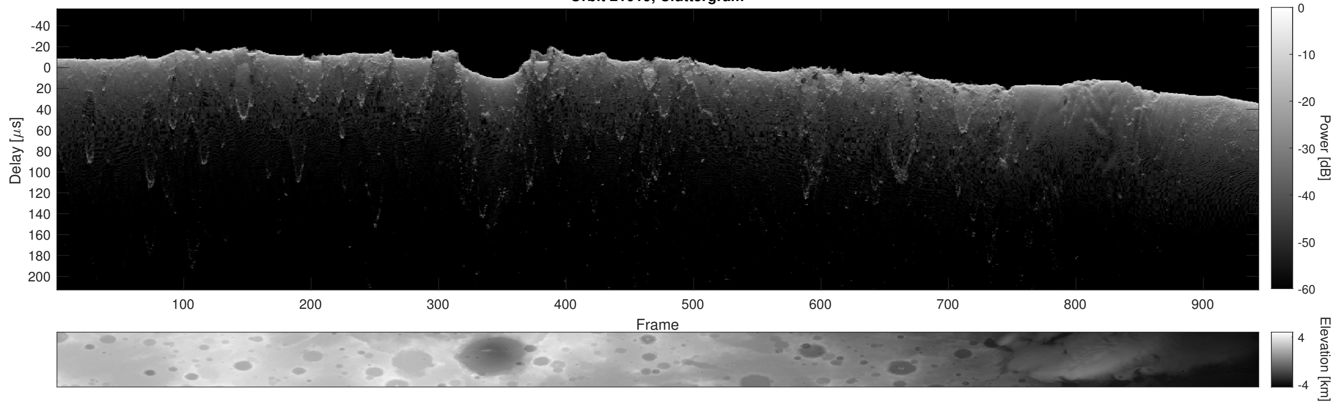
Orbit 21019, Cluttergram
