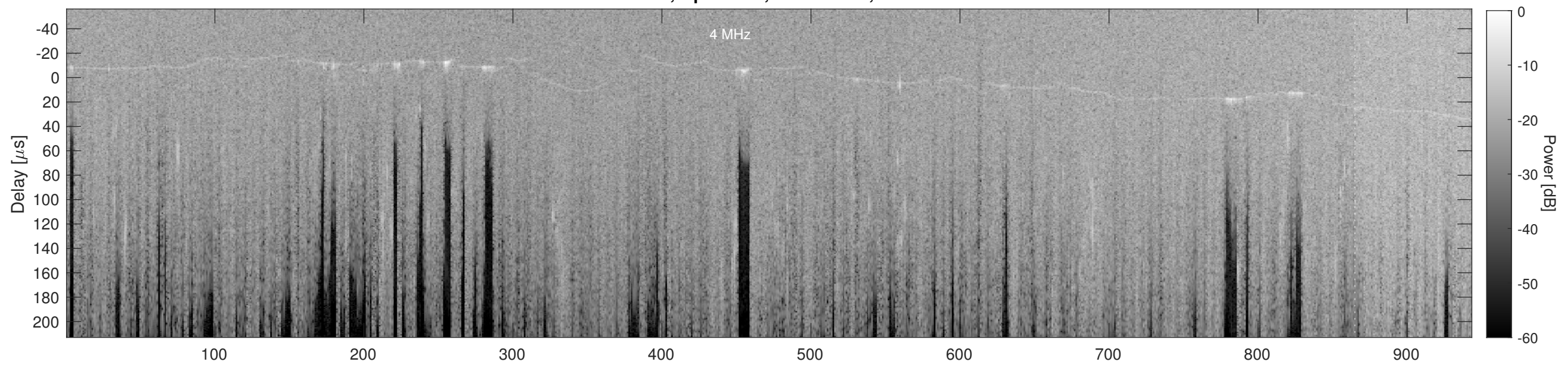
Orbit 21019, Cluttergram
