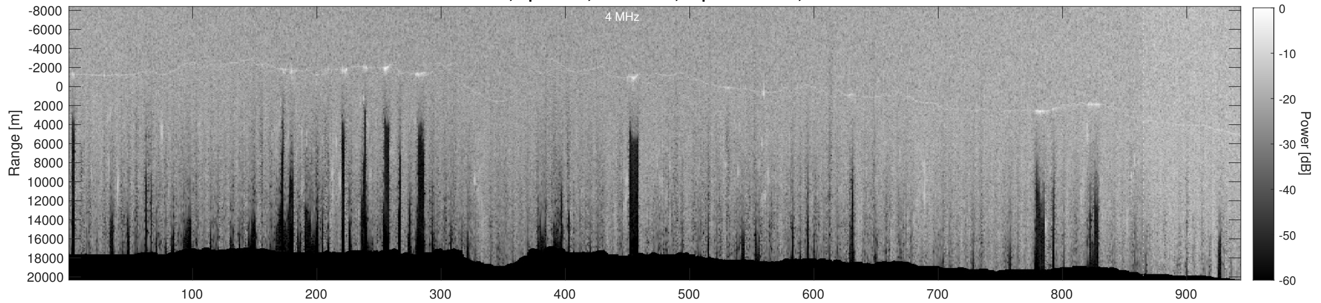
Orbit 21019, Depth-Corrected Cluttergram
