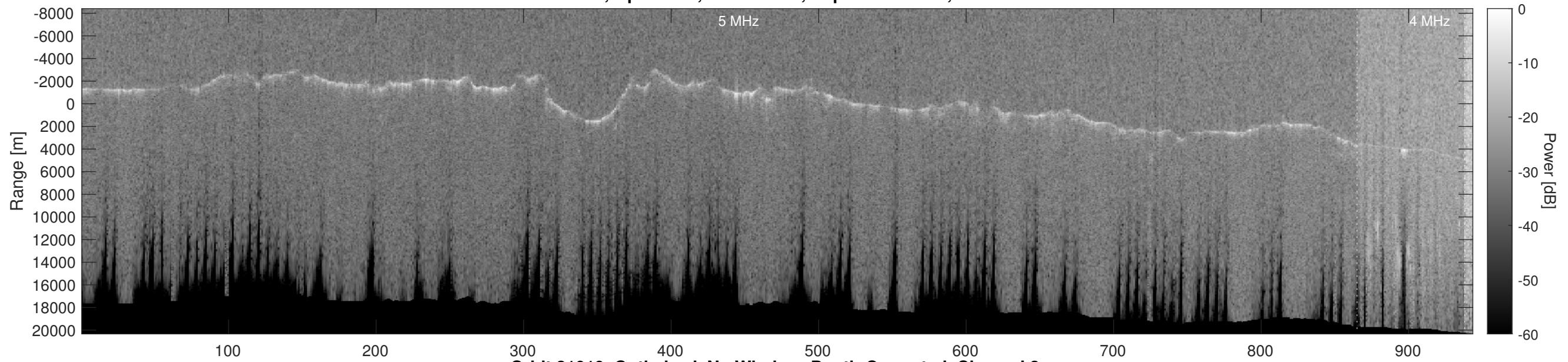
Orbit 21019, Optimized, No Window, Depth-Corrected, Channel 2
