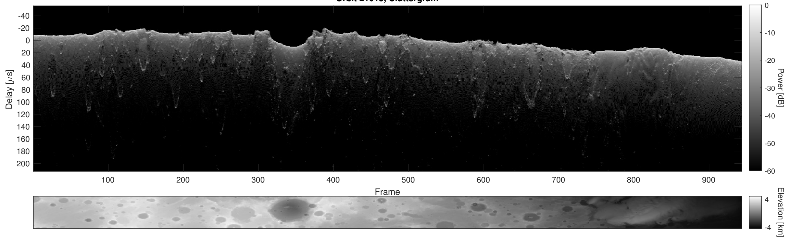
Orbit 21019, Cluttergram
