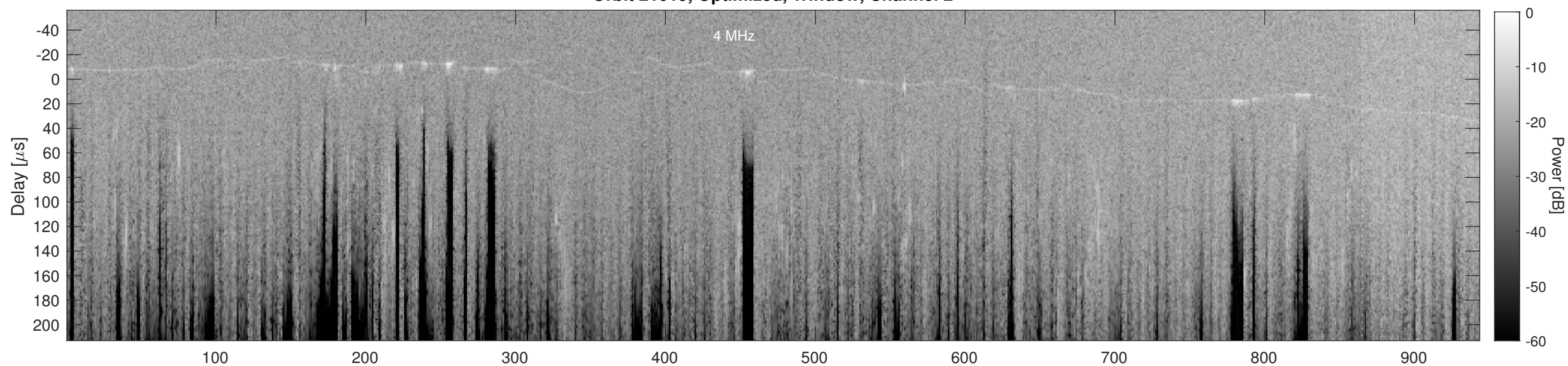
Orbit 21019, Cluttergram
