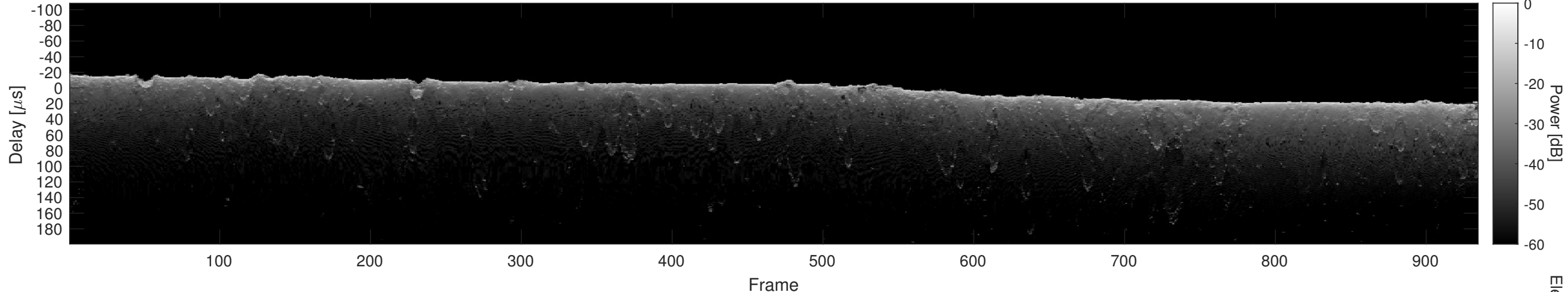
Orbit 21021, Cluttergram
