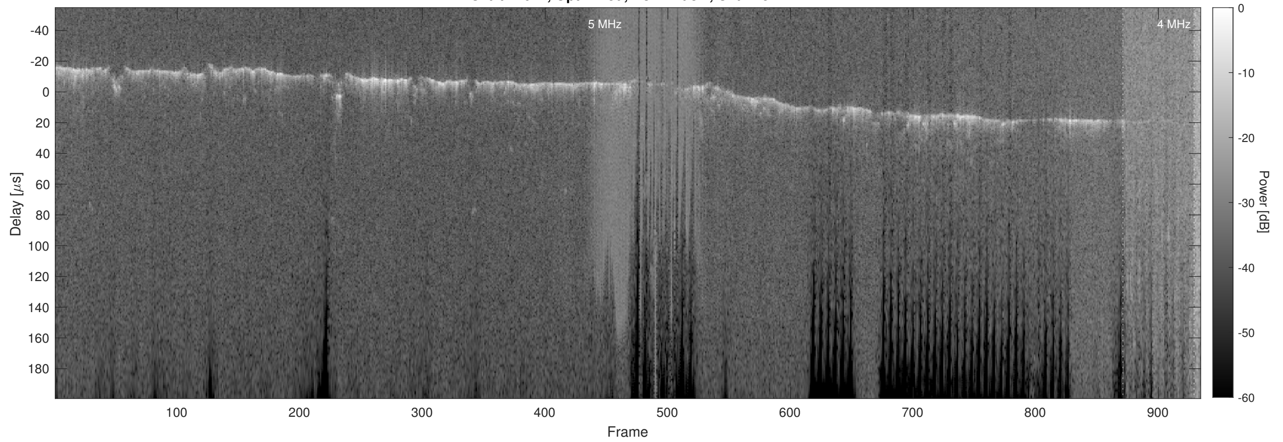
Orbit 21021, Optimized, No Window, Channel 2
