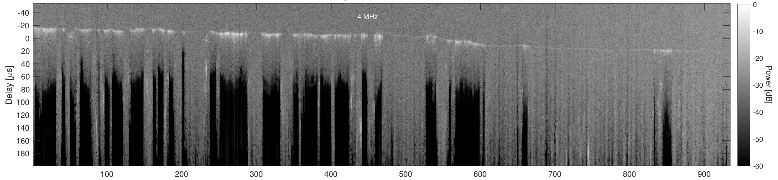
Orbit 21021, Cluttergram
