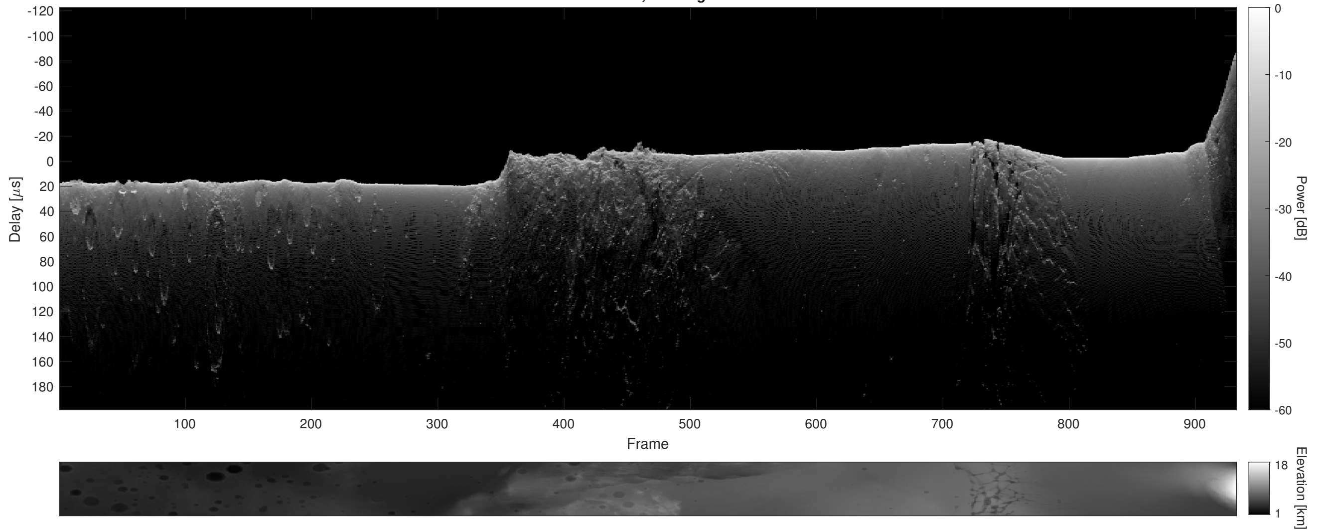
Orbit 21022, Cluttergram
