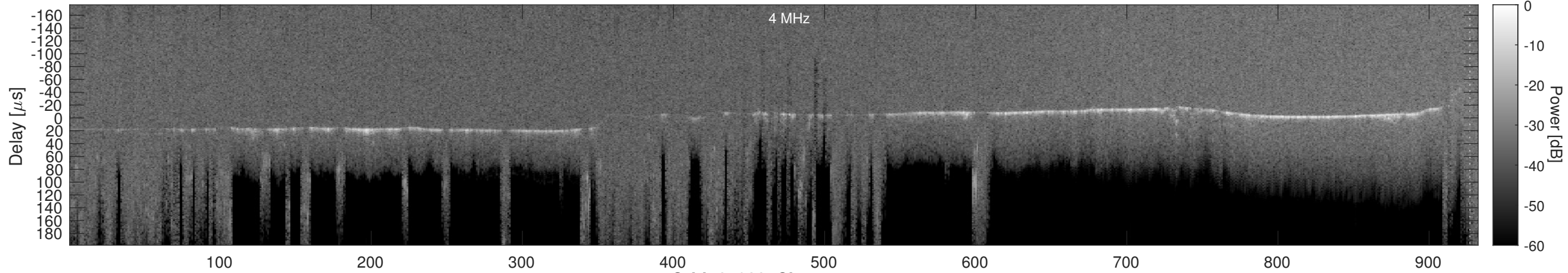
Orbit 21022, Cluttergram
