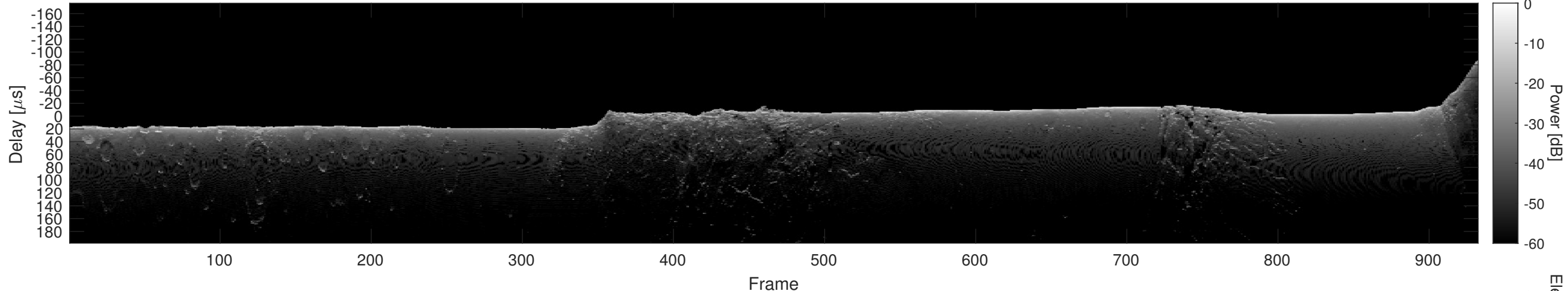
Orbit 21022, Cluttergram
