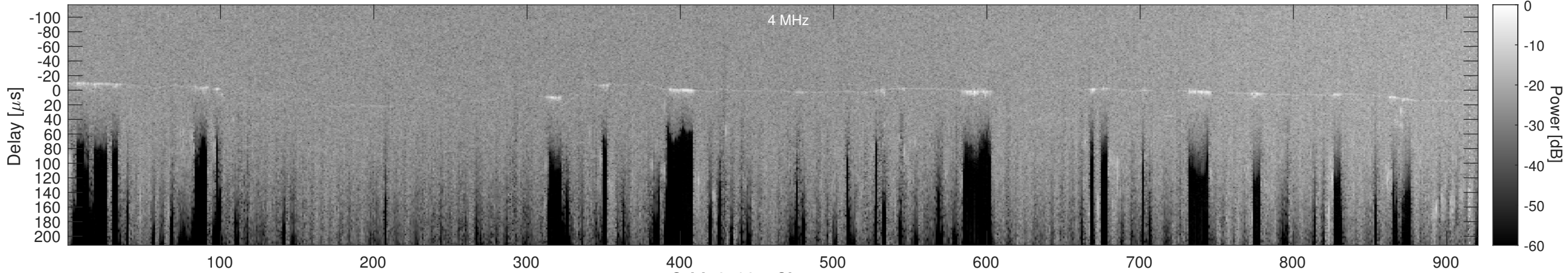
Orbit 21025, Cluttergram
