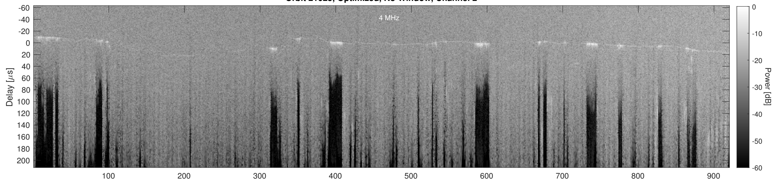
Orbit 21025, Cluttergram
