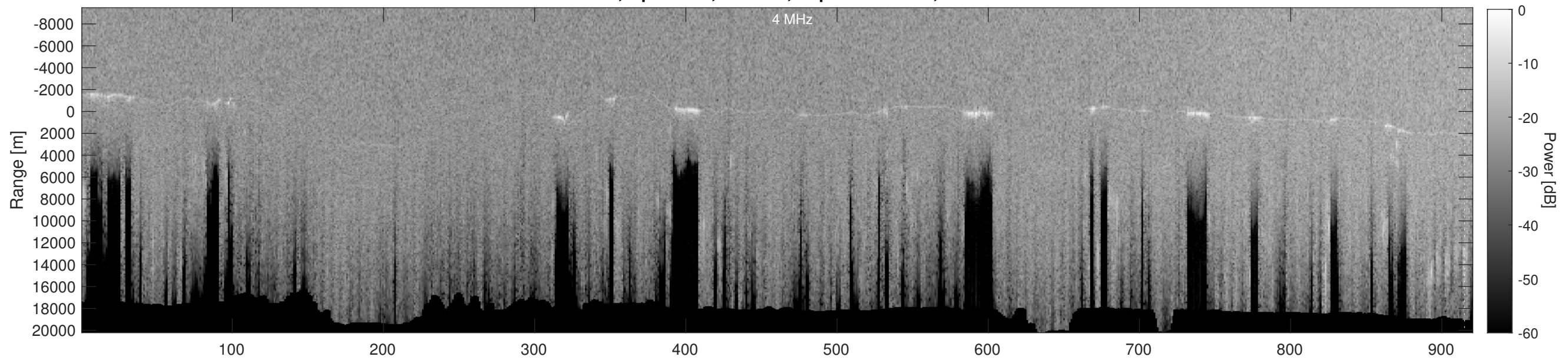
Orbit 21025, Depth-Corrected Cluttergram
