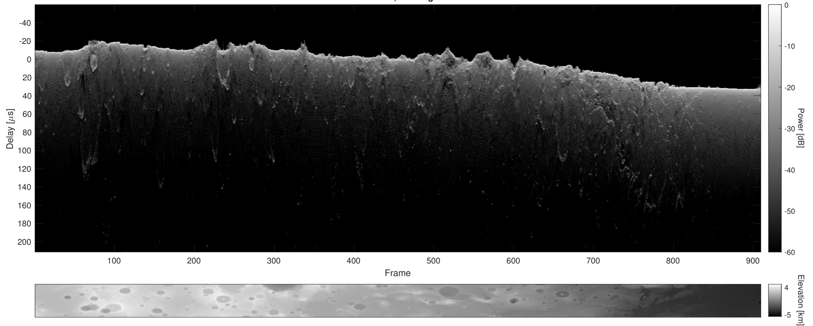
Orbit 21026, Cluttergram
