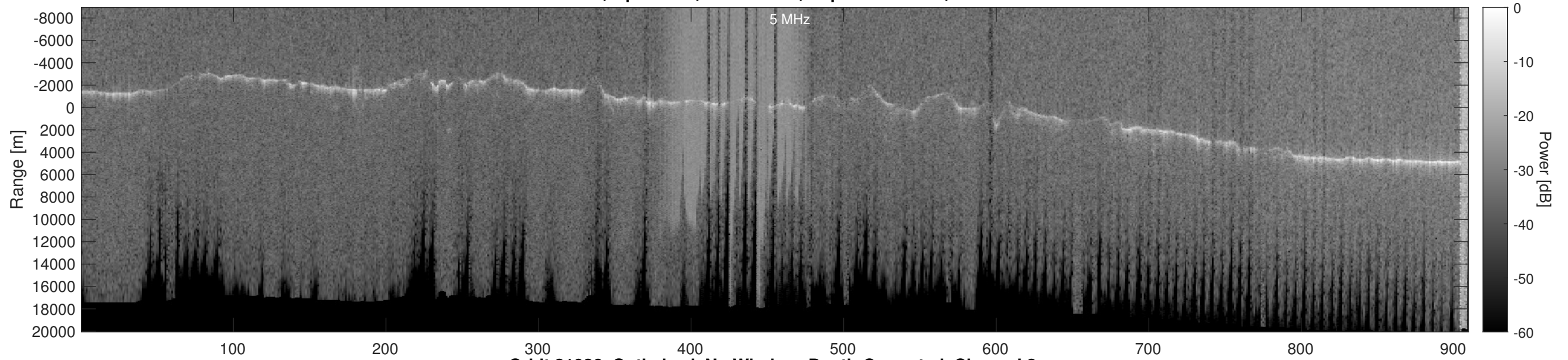
Orbit 21026, Optimized, No Window, Depth-Corrected, Channel 2
