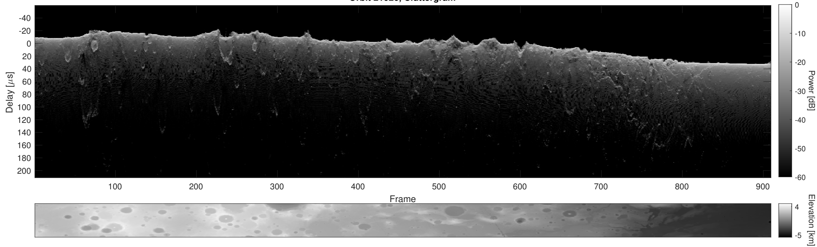
Orbit 21026, Cluttergram
