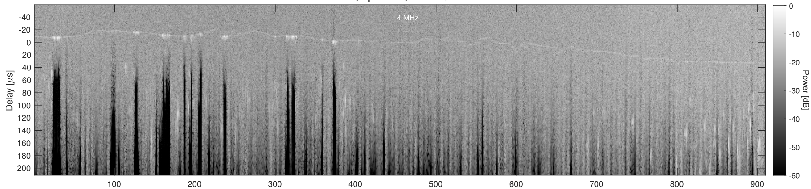
Orbit 21026, Cluttergram
