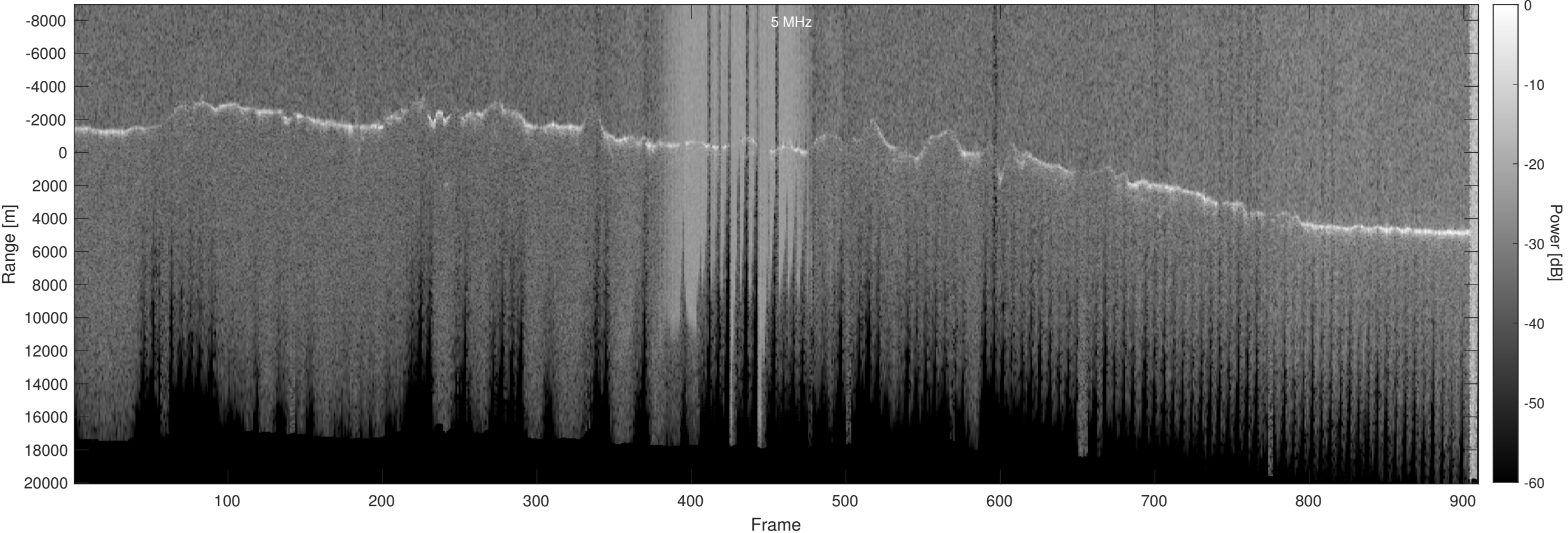
Orbit 21026, Optimized, Window, Depth-Corrected, Channel 2
