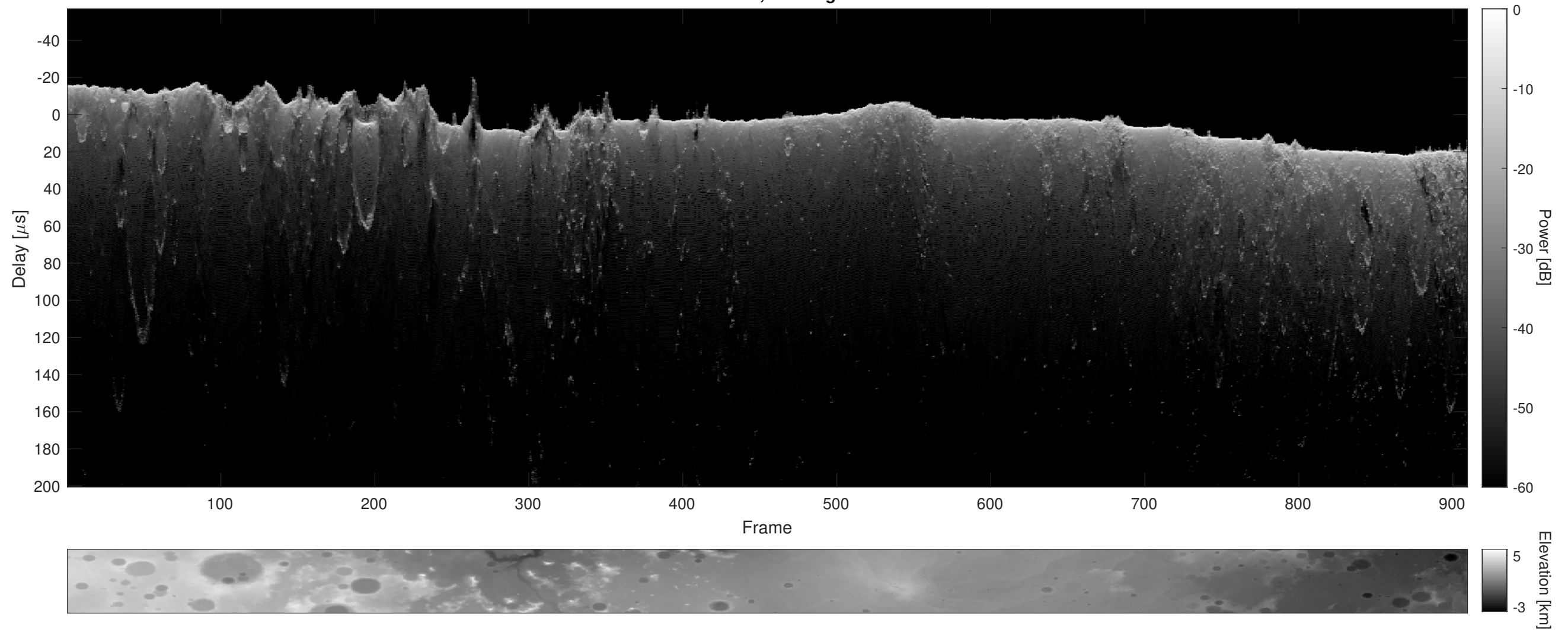
Orbit 21027, Cluttergram
