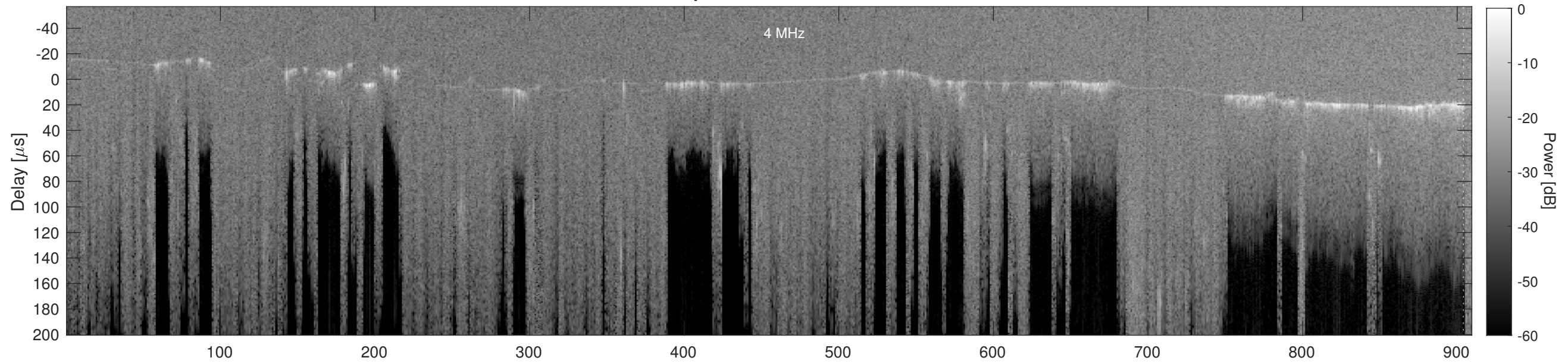
Orbit 21027, Cluttergram
