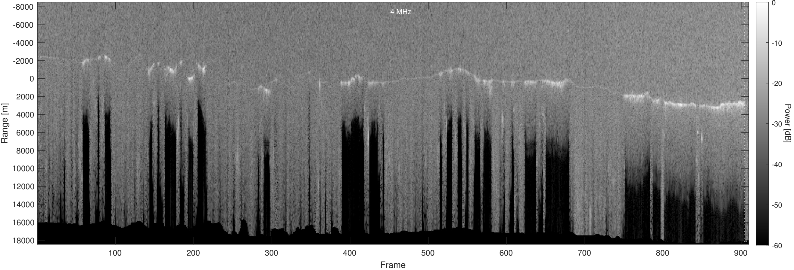
Orbit 21027, Optimized, No Window, Depth-Corrected, Channel 2
