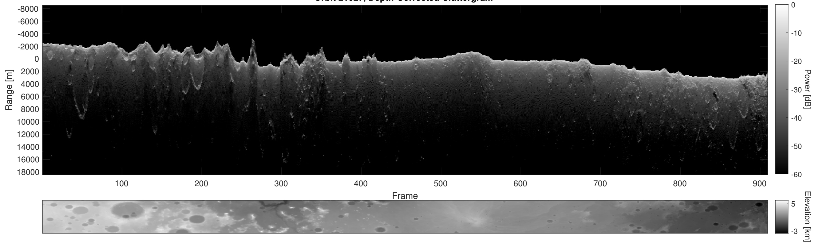
Orbit 21027, Depth-Corrected Cluttergram
