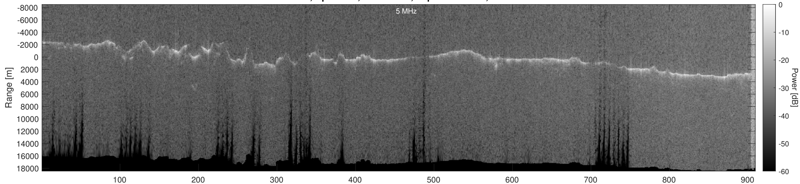
Orbit 21027, Optimized, No Window, Depth-Corrected, Channel 2
