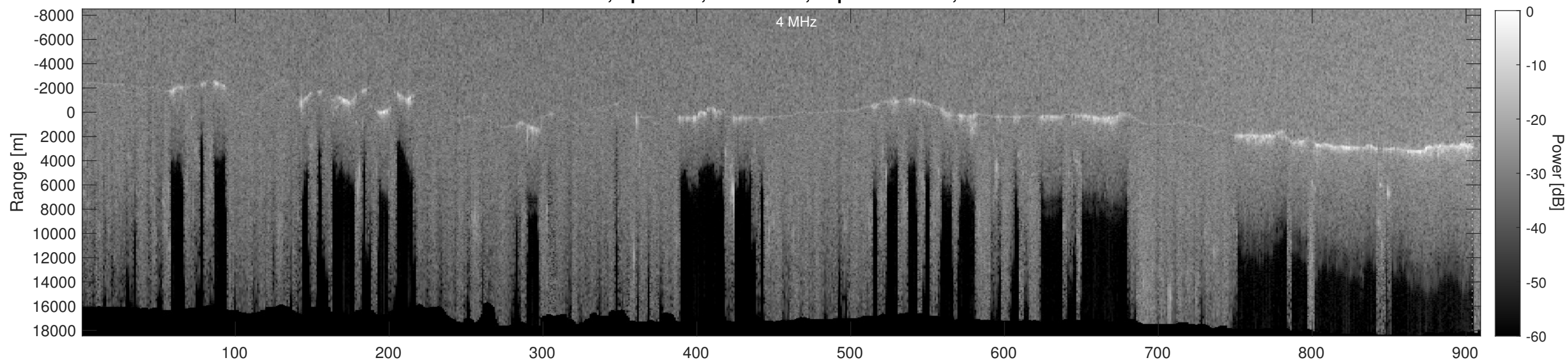
Orbit 21027, Depth-Corrected Cluttergram
