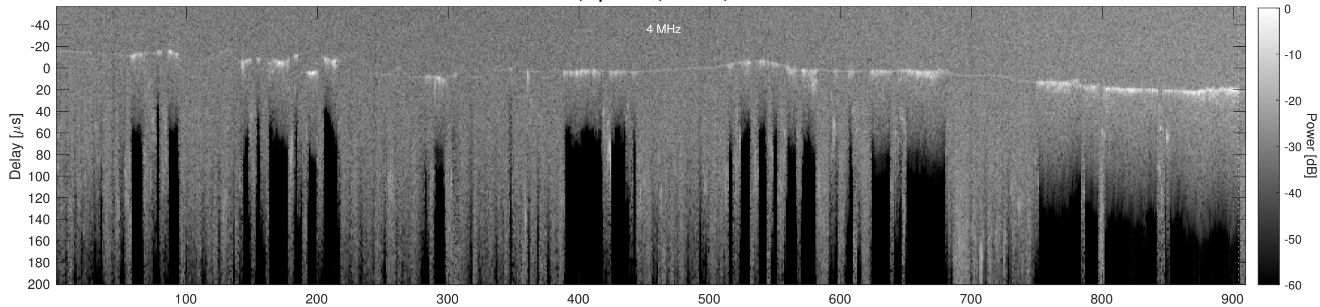
Orbit 21027, Cluttergram
