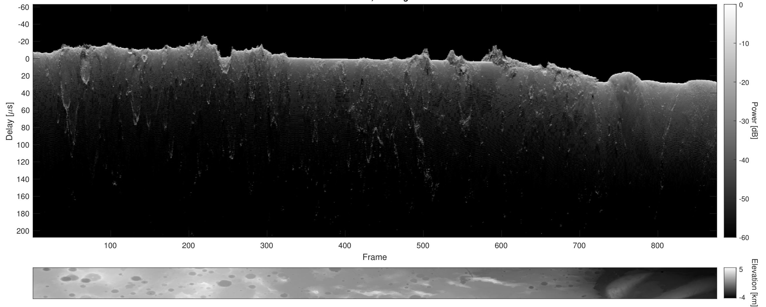
Orbit 21033, Cluttergram
