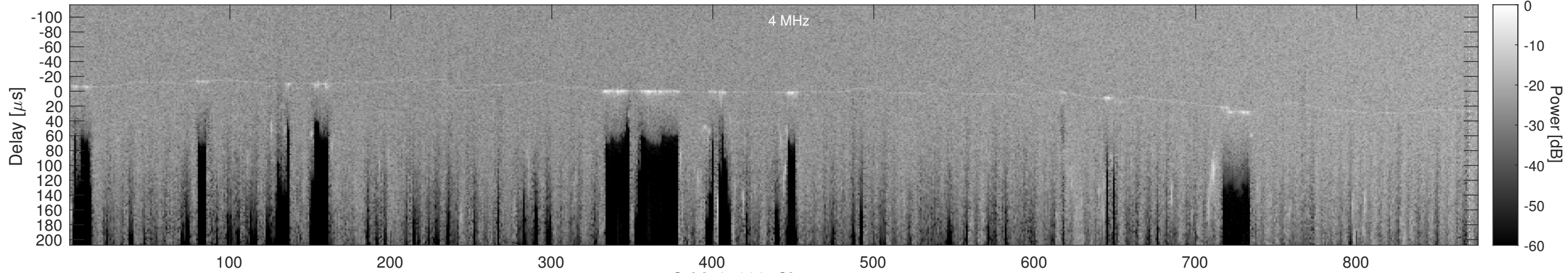
Orbit 21033, Cluttergram
