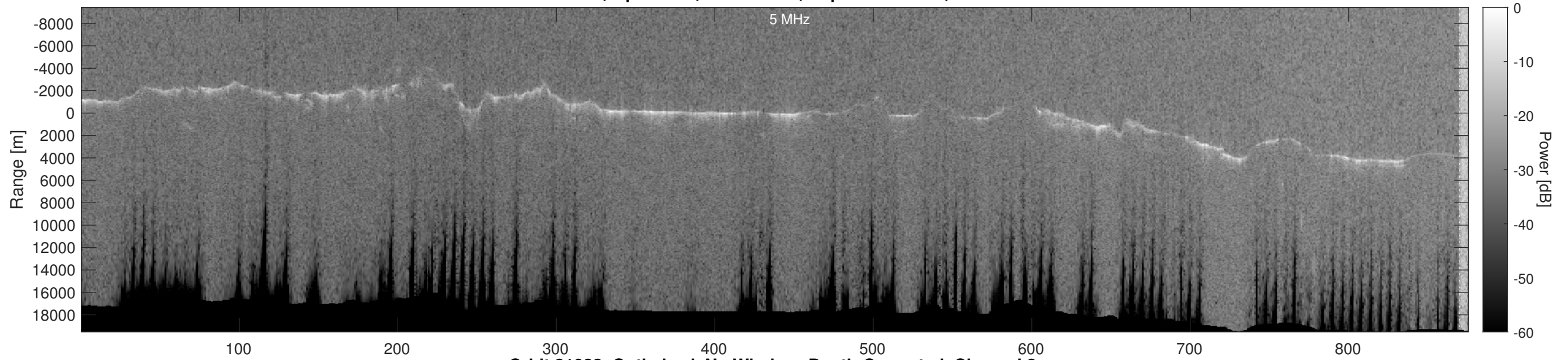
Orbit 21033, Optimized, No Window, Depth-Corrected, Channel 2
