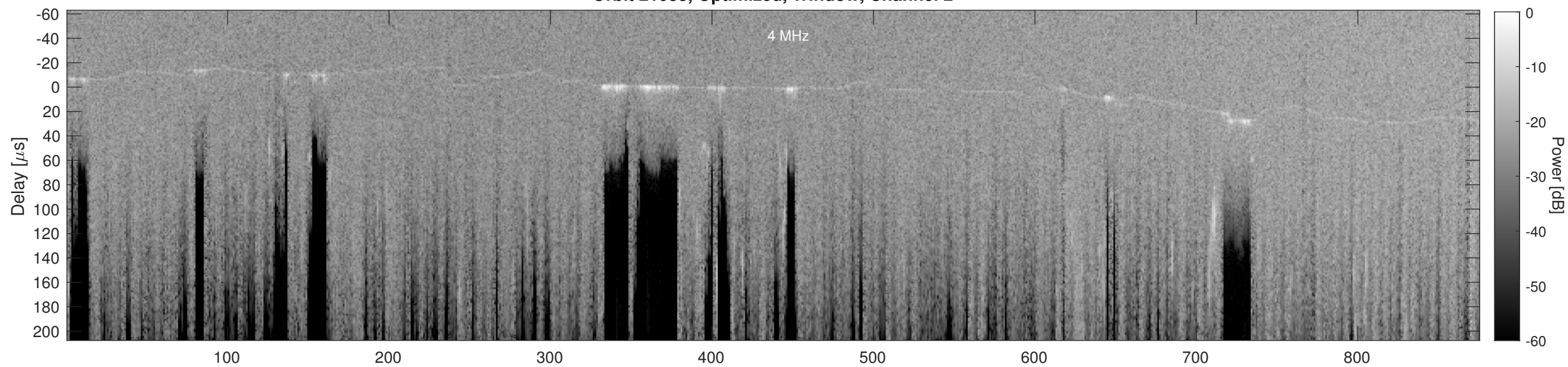
Orbit 21033, Cluttergram
