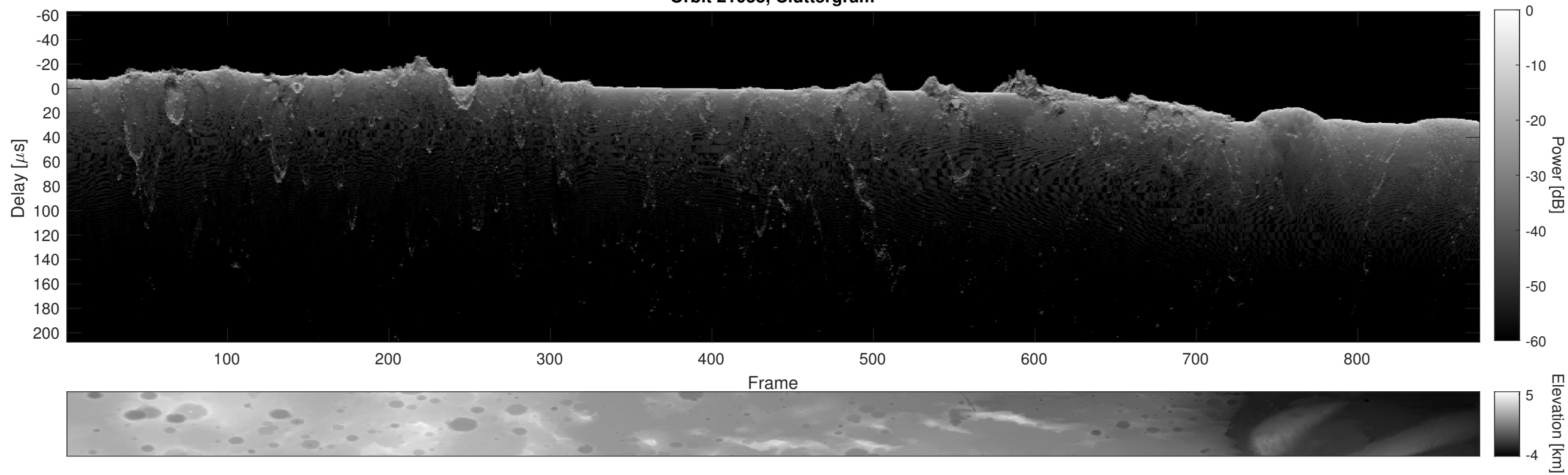
Orbit 21033, Cluttergram
