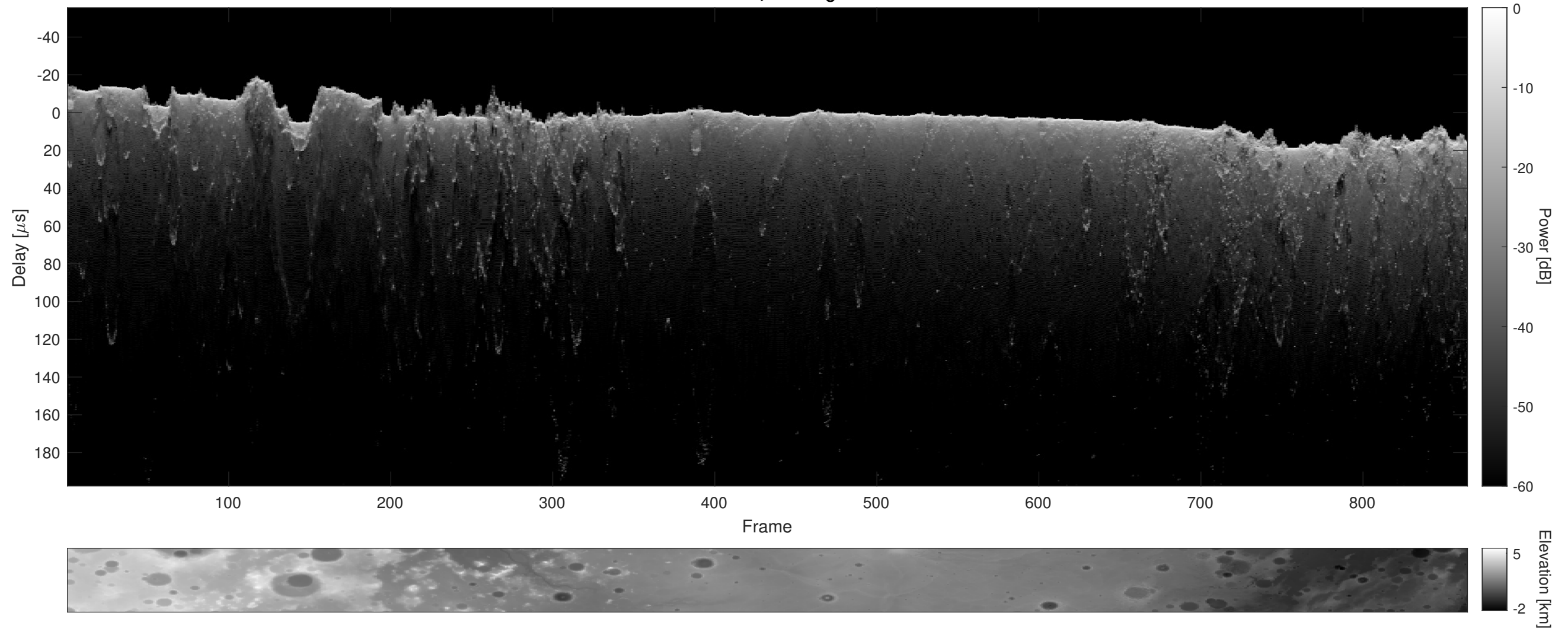
Orbit 21034, Cluttergram
