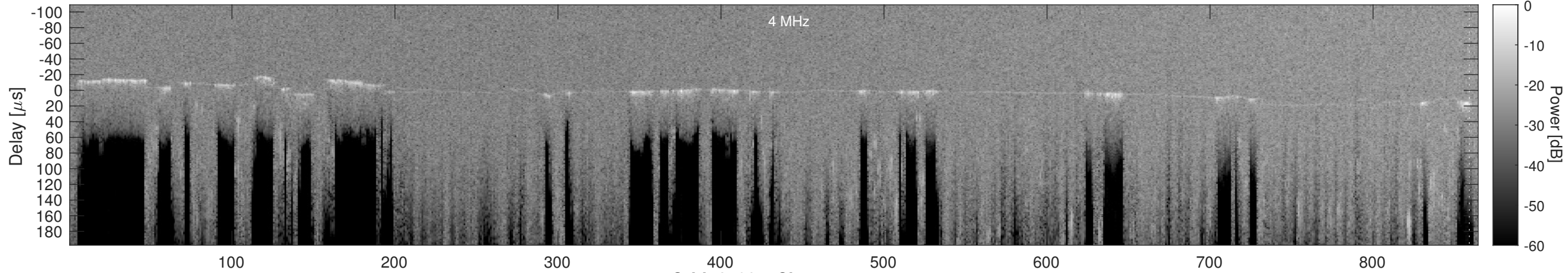
Orbit 21034, Cluttergram
