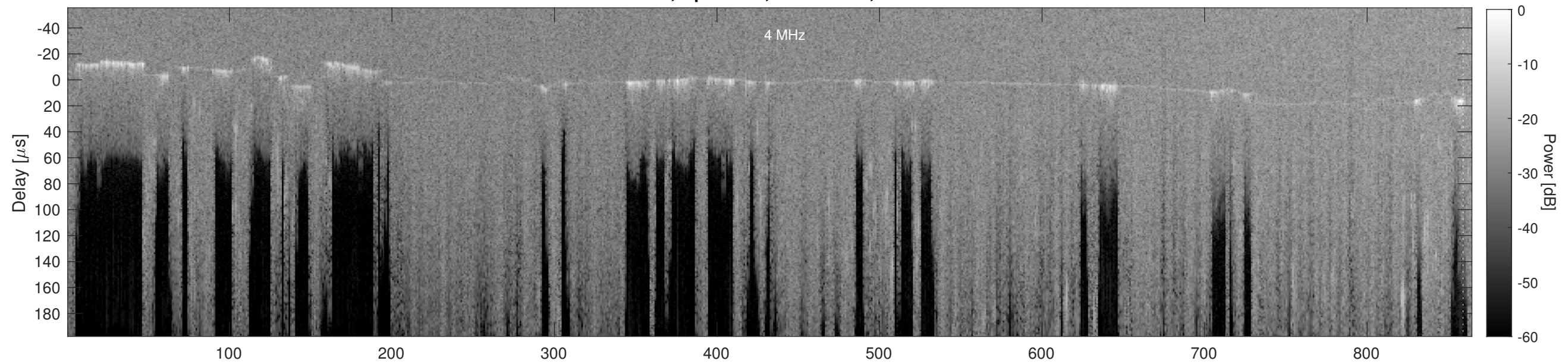
Orbit 21034, Cluttergram
