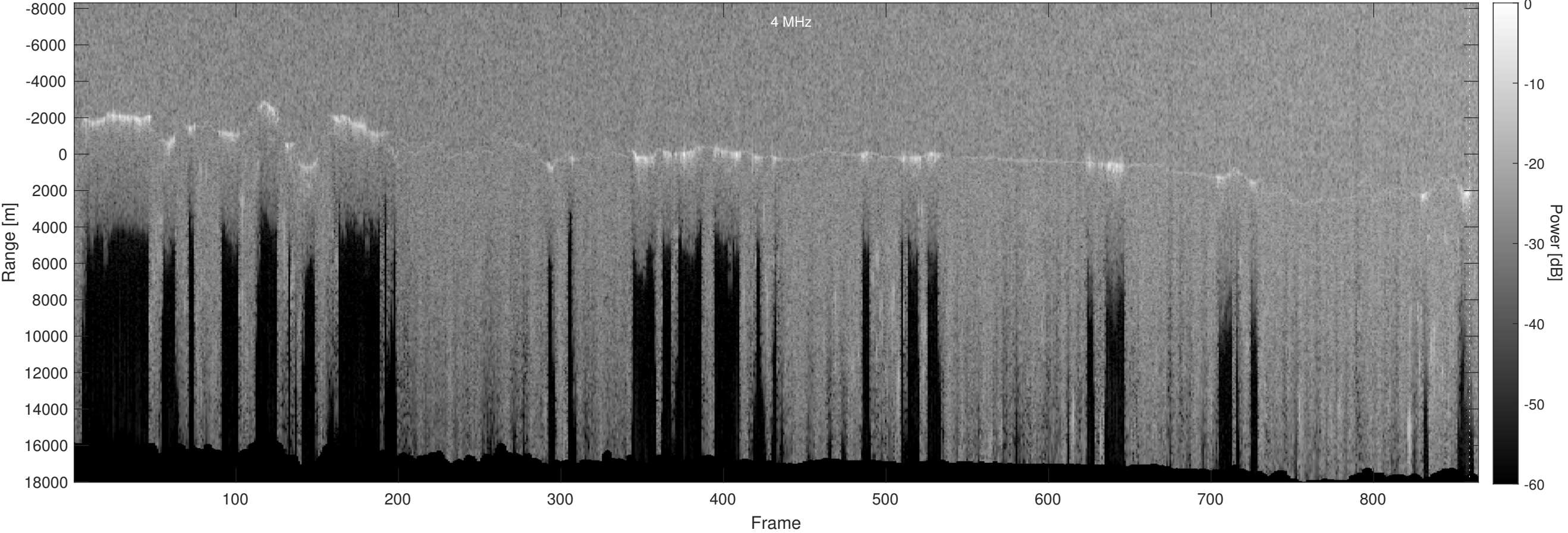
Orbit 21034, Optimized, No Window, Depth-Corrected, Channel 2
