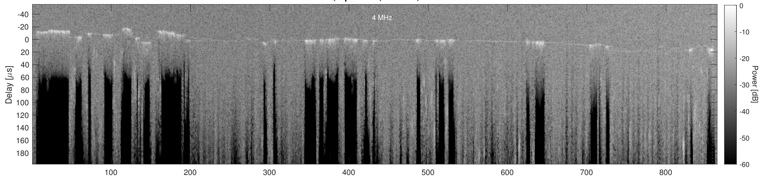
Orbit 21034, Cluttergram
